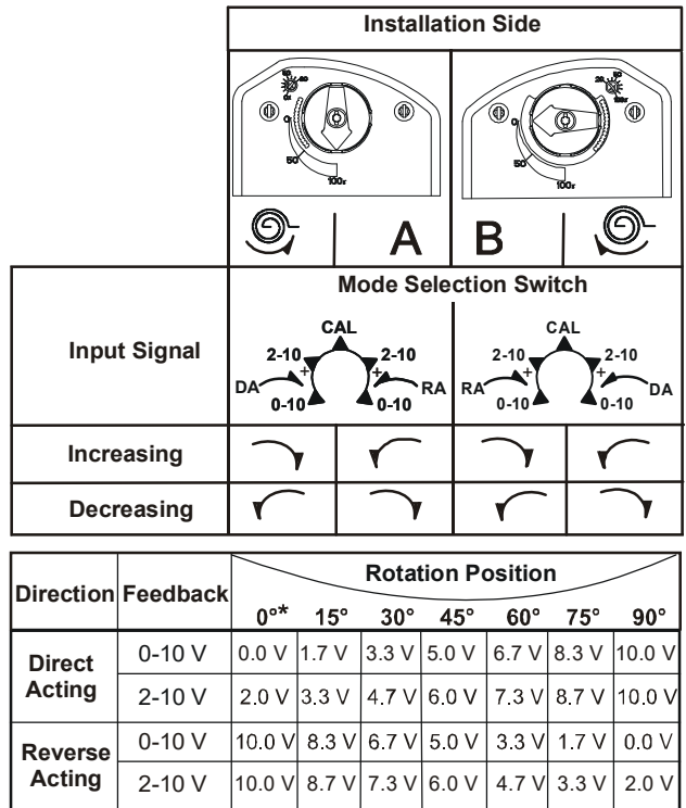
Figure 24: Control response
