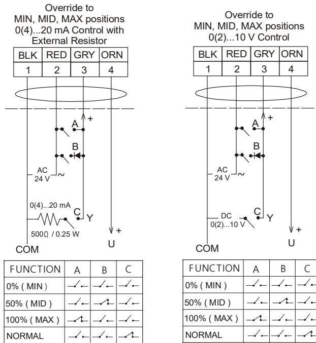
Figure 20: Control wiring diagrams (overrides)
